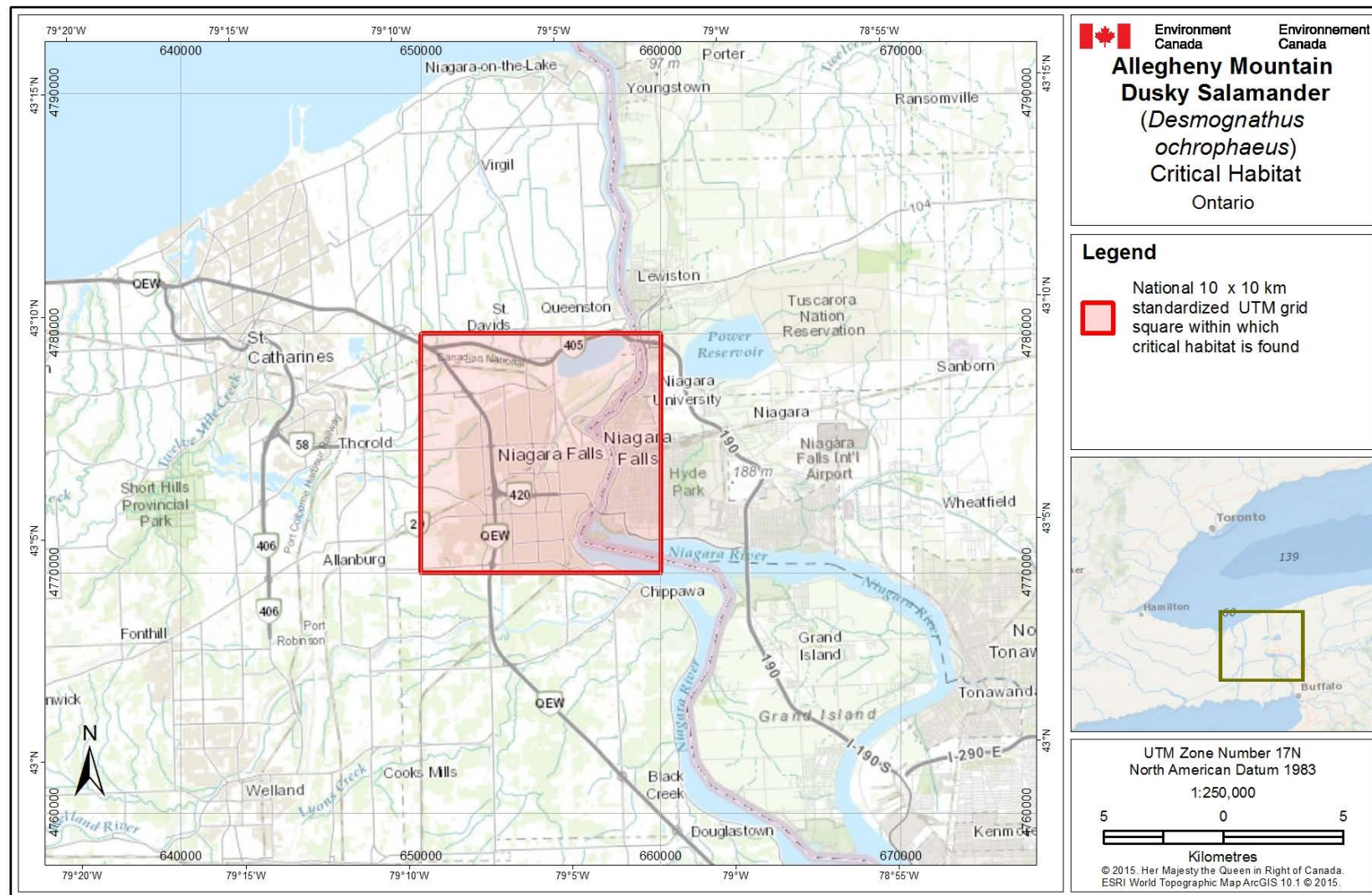
Figure 1. Grid square that contains critical habitat for the Allegheny Mountain Dusky Salamander – Carolinian population in Canada. Critical habitat for the Allegheny Mountain Dusky Salamander occurs within this 10 x 10 km standardized UTM grid square (red square), where the criteria described in Section 6 are met.
